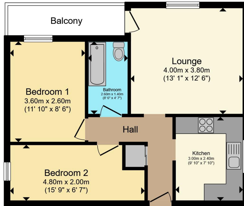
Floor Plan
