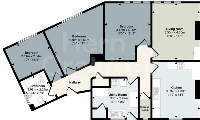
Floorplan
