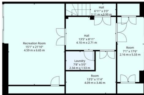
Basement 1
