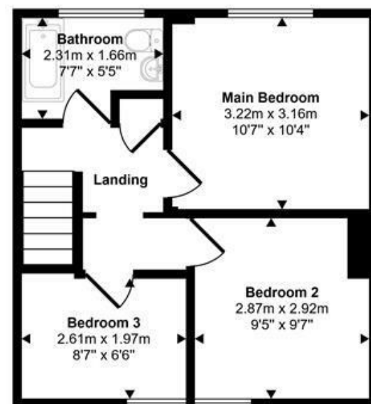
First Floor Approx 35 sq m / 380 sq ft
