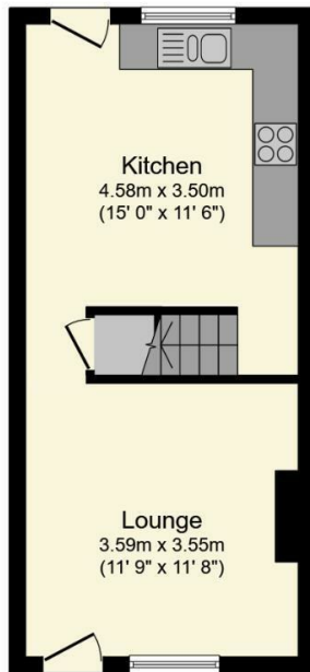
Ground Floor Floor area 29.7 sq.m. (319 sq.ft.)
