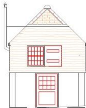
Proposed south elevation
