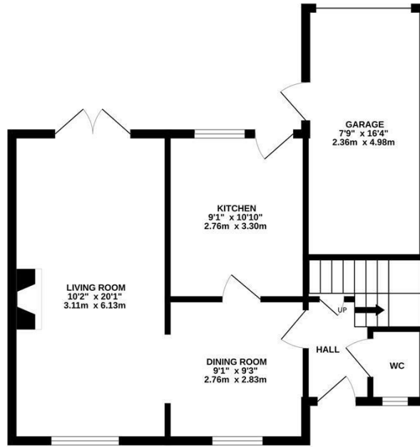
TOTAL FLOOR AREA : 1103 sq.ft. (102.4 sq.m.) approx.
