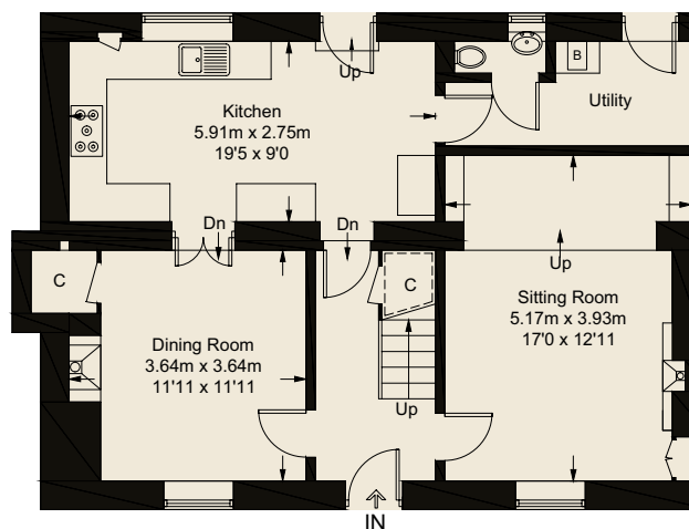
Ground Floor 69.3 sq m / 746 sq ft
