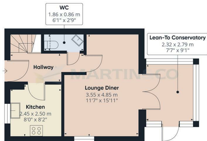
Floor 0
