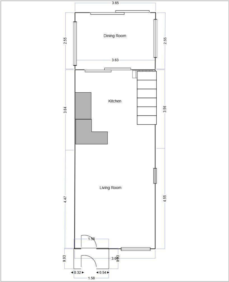
Floor Plan
