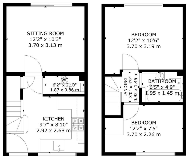
FLOOR 1 FLOOR 2 GROSS INTERNAL AREA TOTAL: 52 m 2 /552 sq ft FLOOR 1: 26 m 2 /277 sq ft, FLOOR 2: 26 m 2 /275 sq ft SIZE AND DIMENSIONS ARE APPROXIMATE, ACTUAL MAY VARY
