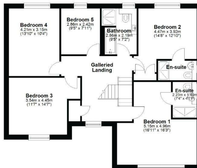
First Floor Approx. 98.4 sq. metres (1059.1 sq. feet)
