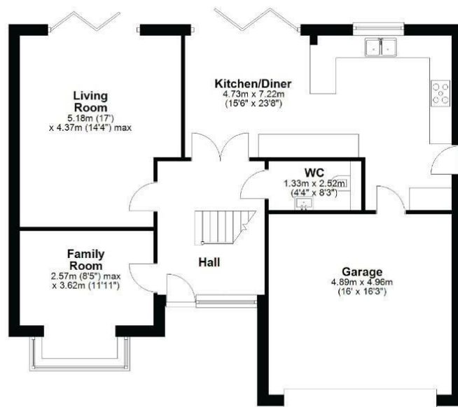
Ground Floor Approx. 99.2 sq. metres (1067.8 sq. feet)
