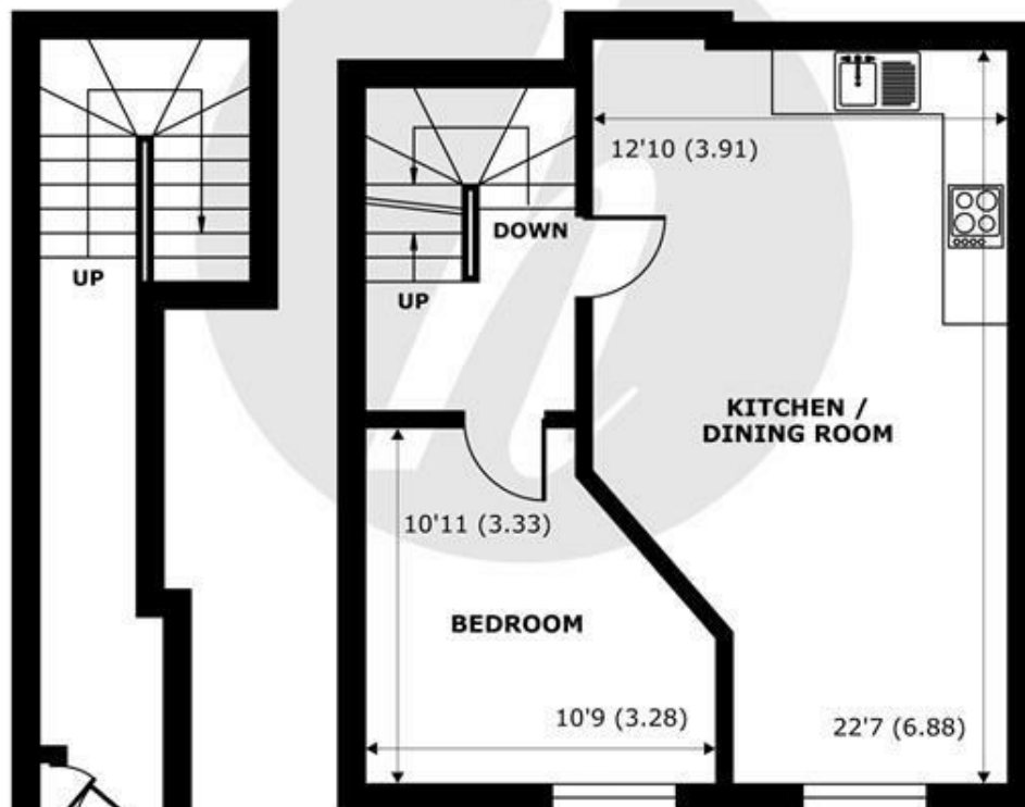
FIRST FLOOR abt 443 SQFT (41.1 SQMT)
