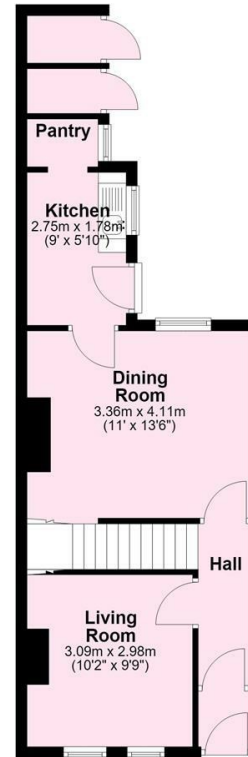
Ground Floor Approx. 39.1 sq. metres (421.3 sq. feet)
