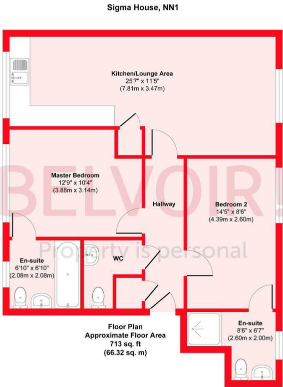
Approx. Gross Internal Floor Area 713 sq. ft / 66.32 sq. m Illustration for identification purposes only, measurements are approximate, not to scale. Produced by Elements Property
