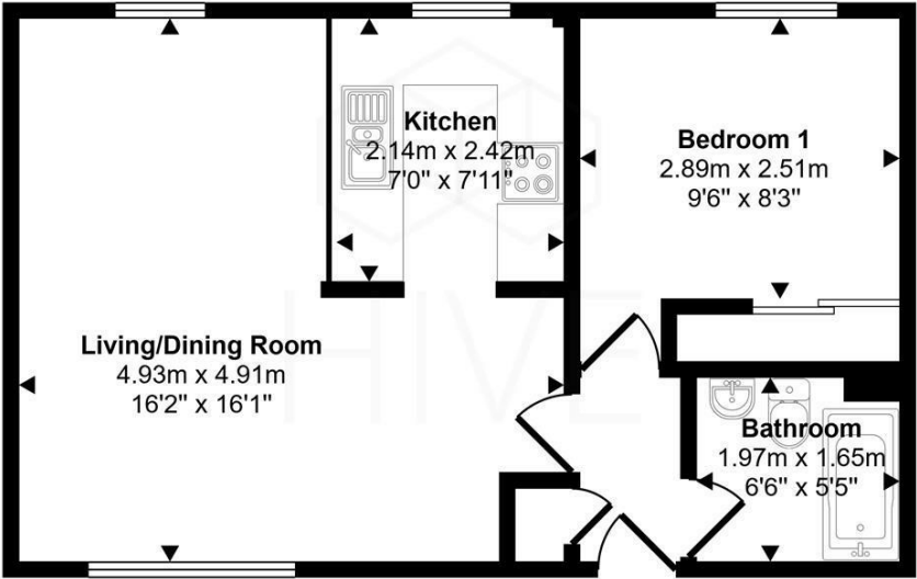
Floorplan
