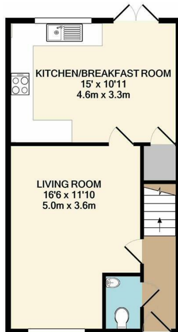
GROUND FLOOR APPROX. FLOOR AREA 412 SQ.FT. (38.2 SQ.M.)
