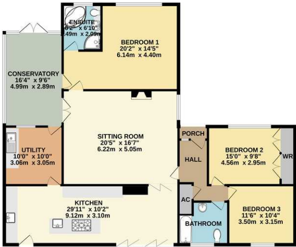
GROUND FLOOR 1576 sq.ft. (146.4 sq.m.) approx.
