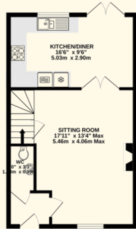
GROUND FLOOR 694 sq.ft. (64.5 sq.m.) approx.
