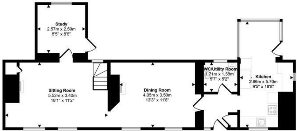
Ground Floor Approx 67 sq m / 727 sq ft
