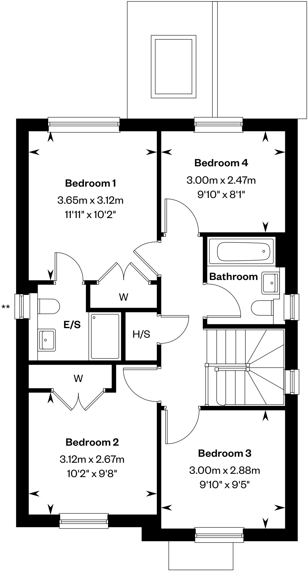
First floor
