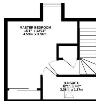
2ND FLOOR
