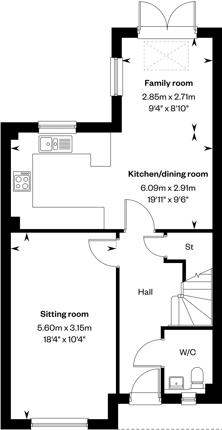
Ground floor
