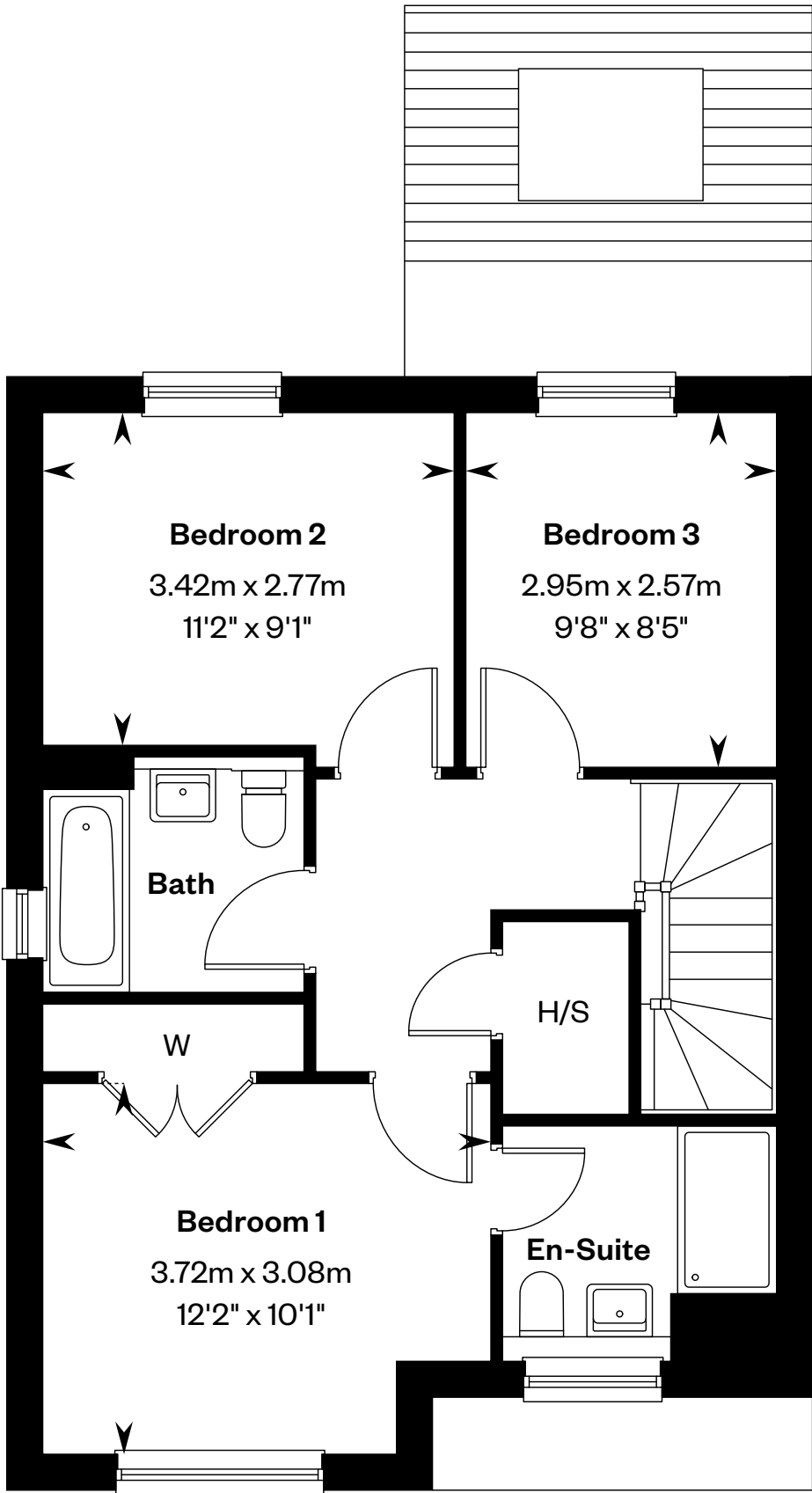
First floor
