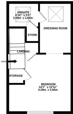
2ND FLOOR 340 sq.ft. (31.6 sq.m.) approx.
