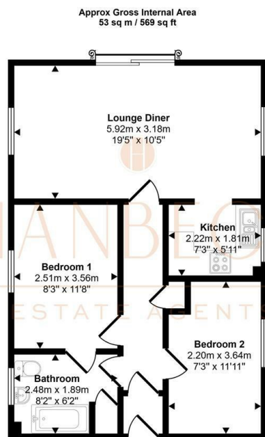
Floorplan
