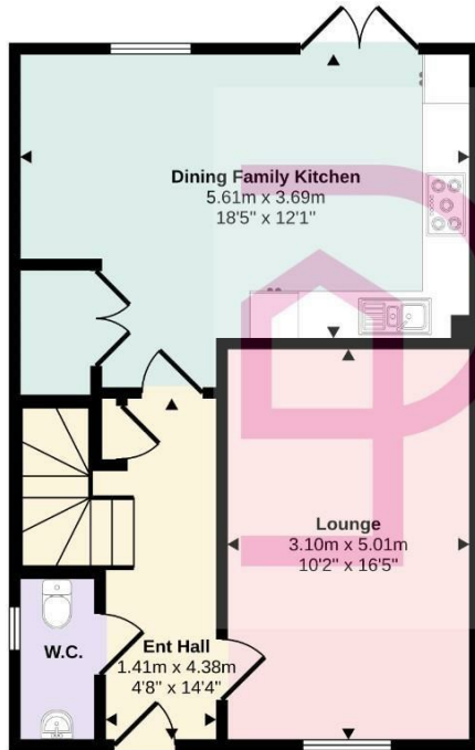
Ground Floor Approx 50 sq m / 540 sq ft
