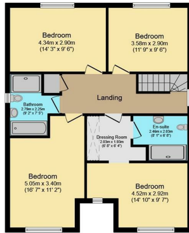
First Floor Floor area 77.2 sq.m. (831 sq.ft.)
