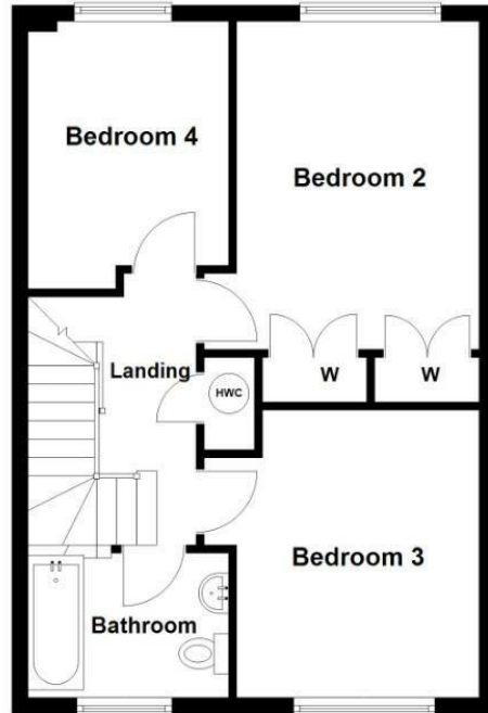
First Floor Approx. 47.7 sq. metres (513.5 sq. feet)
