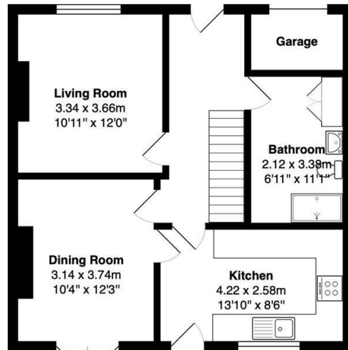
Ground Floor Area: 56.9 m 2 ... 612 ft 2
