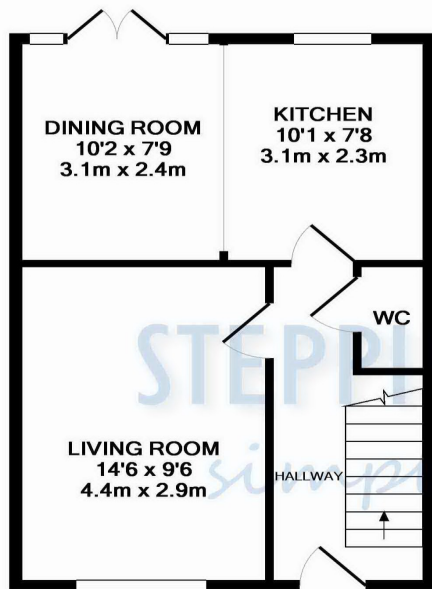
GROUND FLOOR APPROX. FLOOR AREA 380 SQ.FT. (35.3 SQ.M.)
