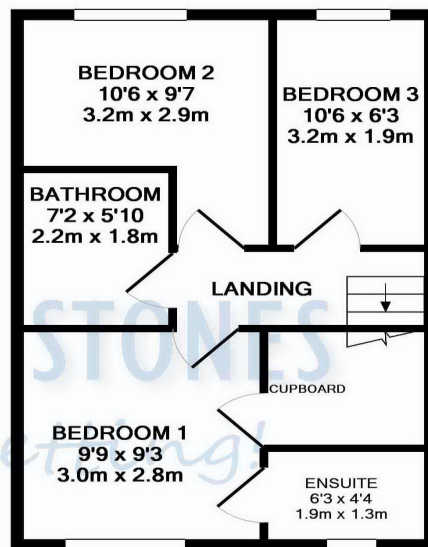
1ST FLOOR APPROX. FLOOR AREA 368 SQ.FT. (34.2 SQ.M.)
