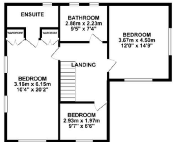
1ST FLOOR 64.81 sq. m. ( 697.61 sq. ft. )
