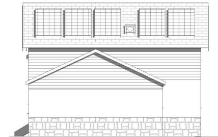
4 South Elevation 1 : 100
