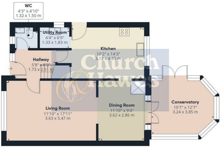
Floor 0 Building 1
