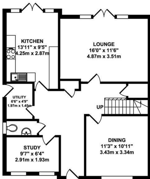
GROUND FLOOR APPROX. FLOOR AREA 741 SQ.FT. 68.85 SQ.M.
