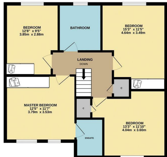
1ST FLOOR 735 sq.ft. (68.3 sq.m.) approx.
