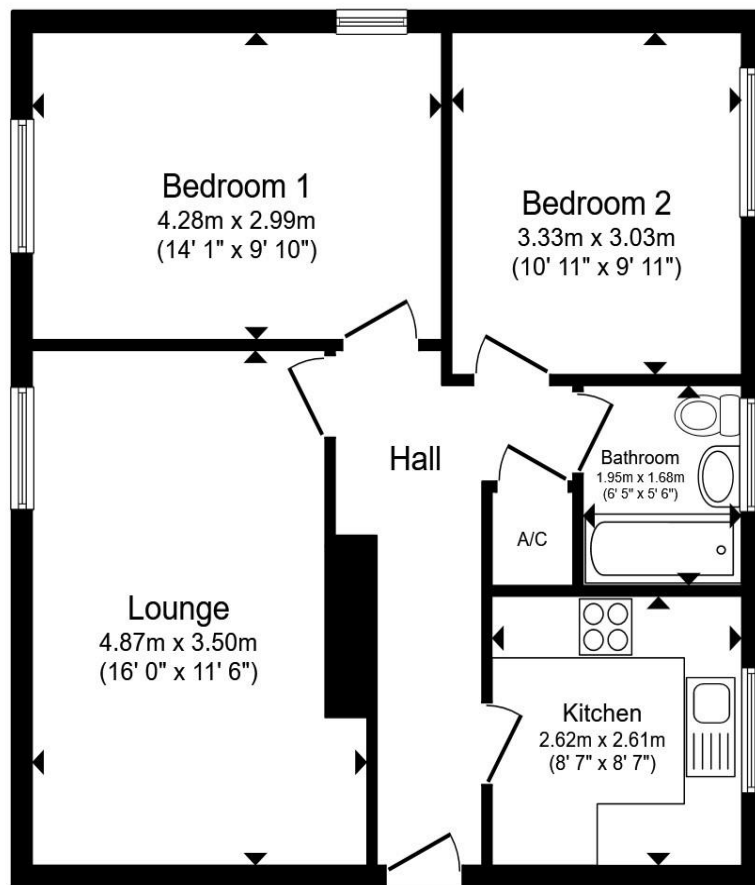
Floor Plan
