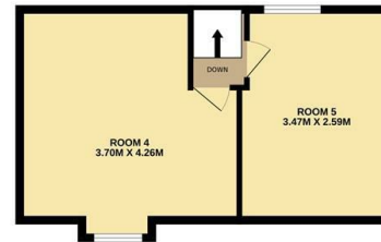
2ND FLOOR
