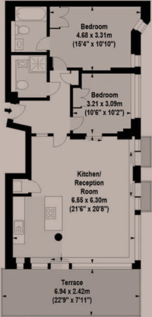
Seventh Floor
