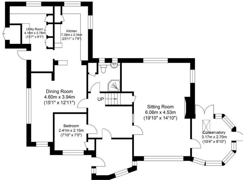
Ground Floor Approximate Floor Area 963.58 sq ft (89.52 sq m)
