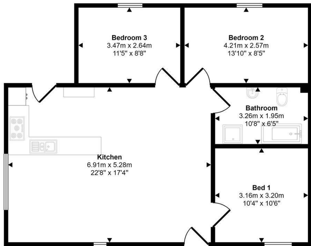
Floorplan
