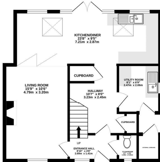
GROUND FLOOR 587 sq.ft. (54.5 sq.m.) approx.
