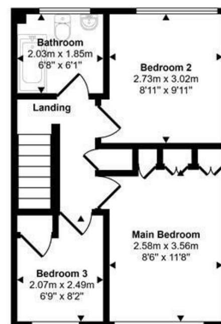
First Floor Approx 35 sq m / 377 sq ft
