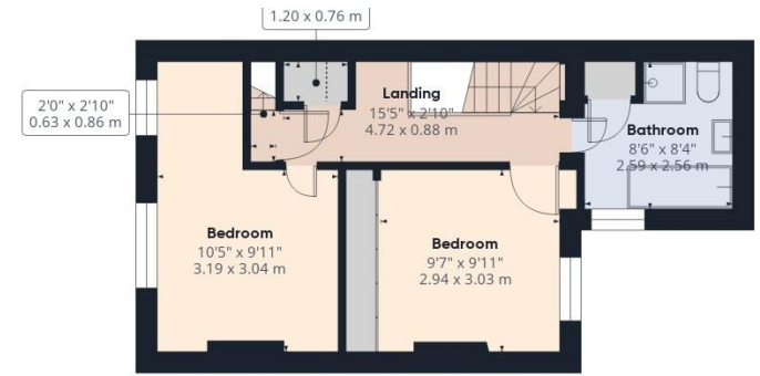
Floor 1
