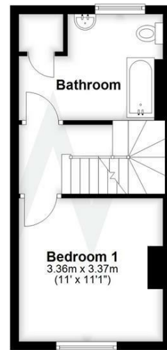
First Floor Approx. 25.9 sq. metres (278.8 sq. feet)
