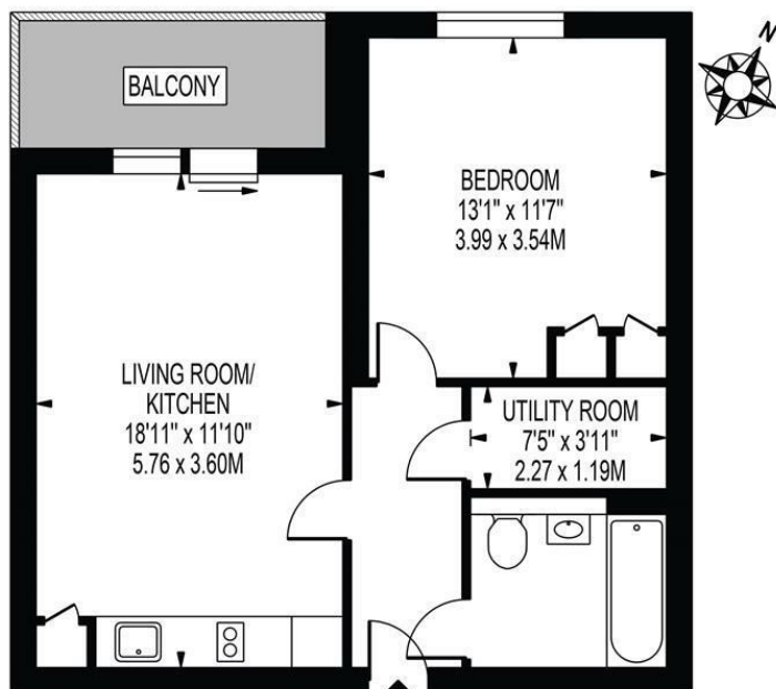
THIRD FLOOR FOR ILLUSTRATION PURPOSES ONLY
