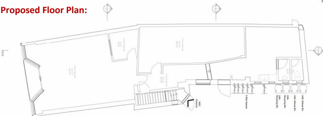
Proposed Ground Floor Plan 1 : 50
