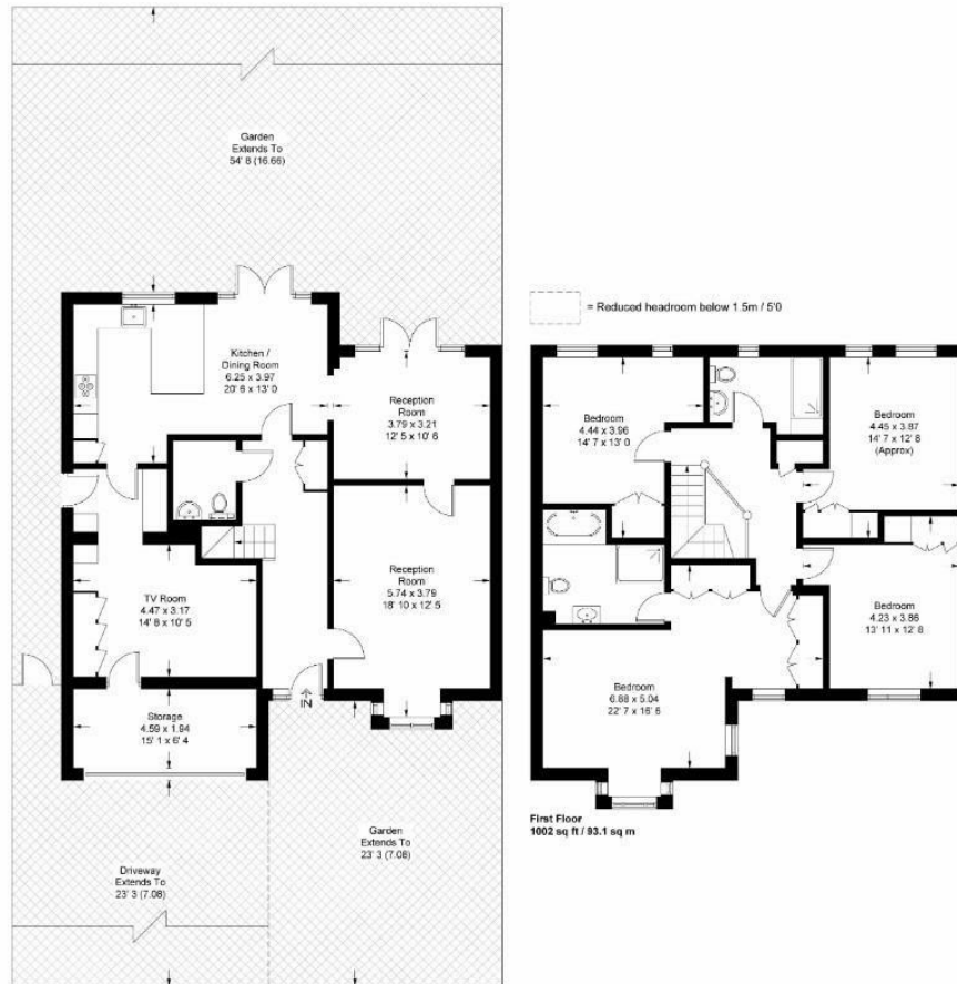
Ground Floor 1102 sq ft / 102.4 sq m (Including Reduced Headroom)
