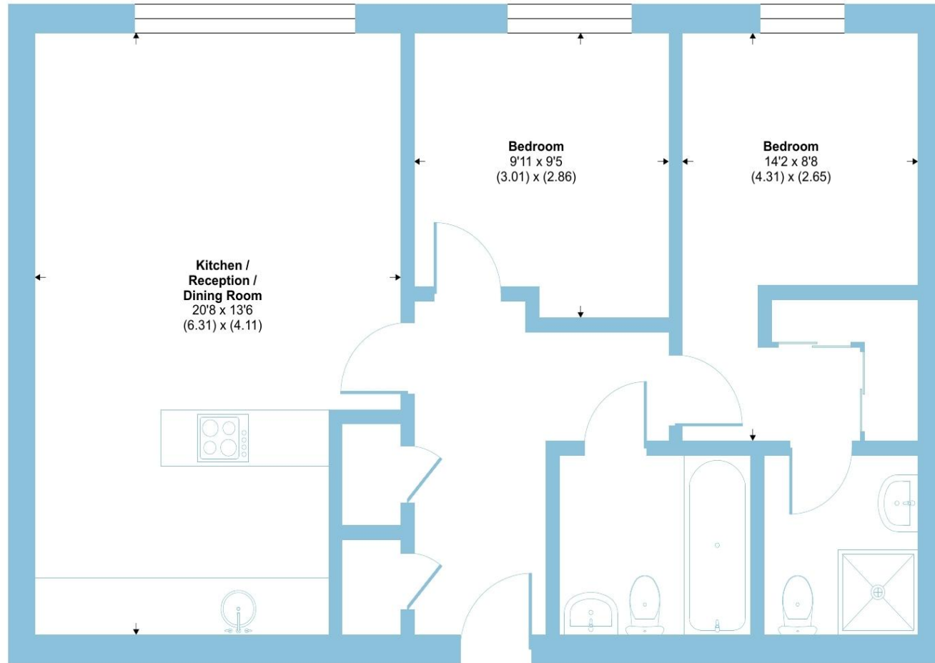
SECOND FLOOR
