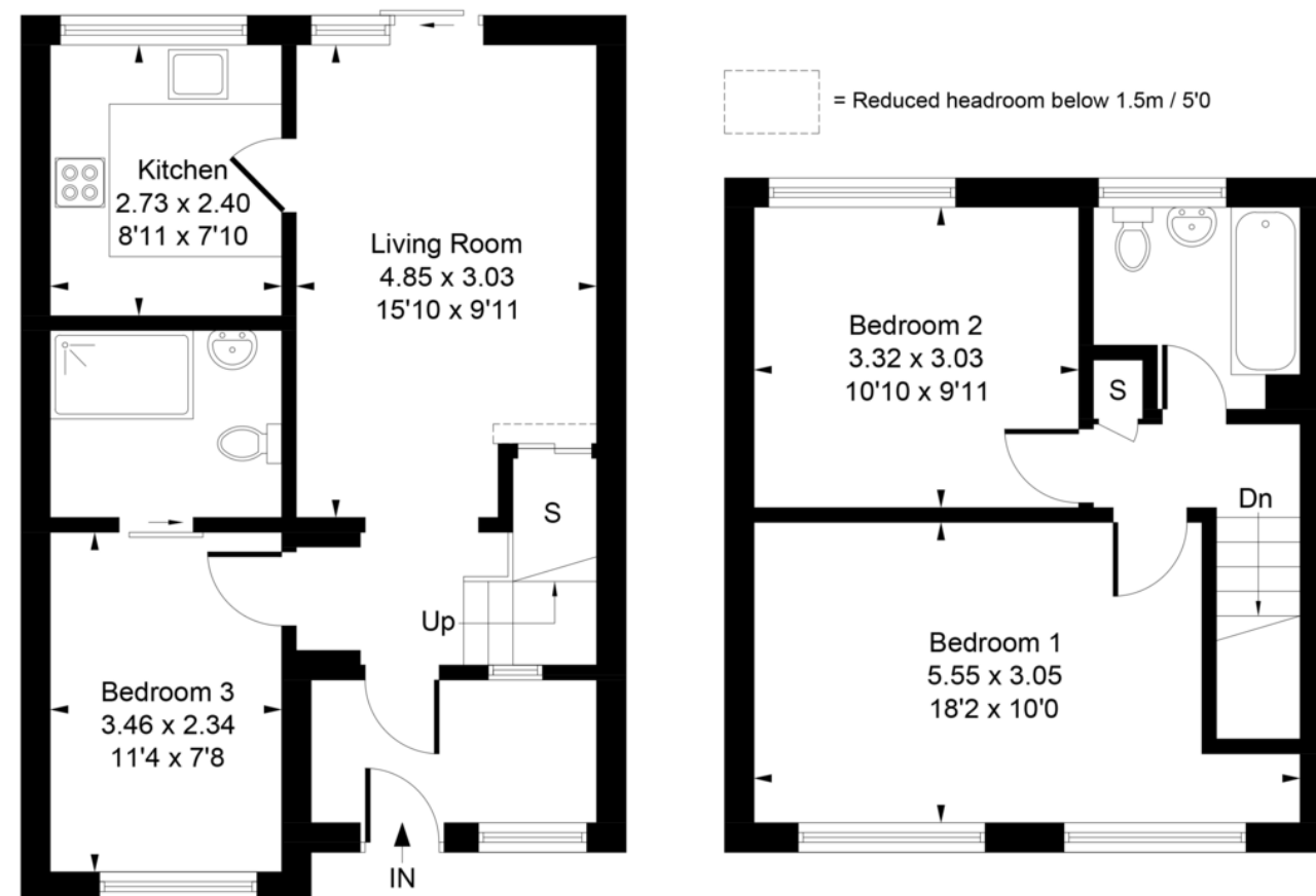
Ground Floor
