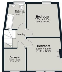
First Floor Approx. 42.6 sq. metres (459.0 sq. feet)
